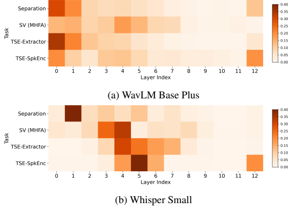
Fig. 2: The weight distribution of Transformer layers. Note that 0-th Transformer layer denotes the output of the CNN encoder, which is also the input of the 1-st Transformer layer.
